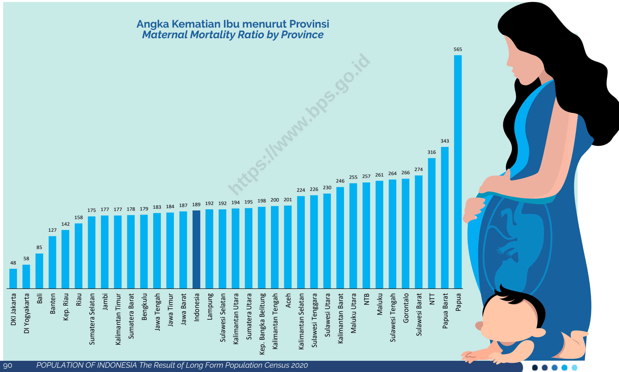
Gambar 5.1 Angka Kematian Ibu menurut Provinsi Figure 5.1 Maternal Mortality Ratio by Province
